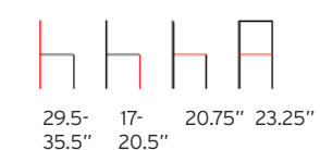
6000 Height Adjustable
